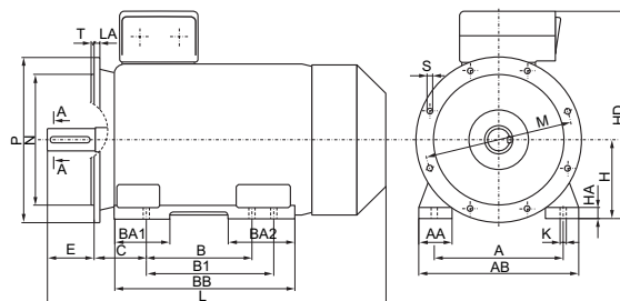
B35, motorstorlek 200–355
