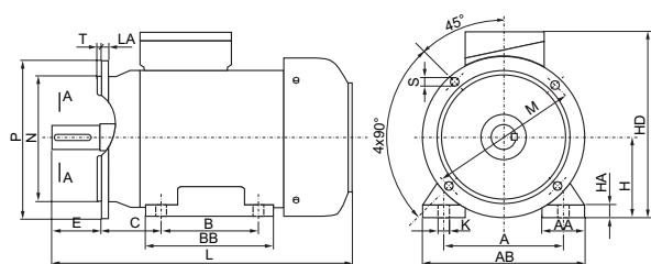
B35, motorstorlek 80–180
